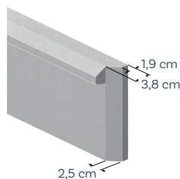
Compatible poteau Ritmo
